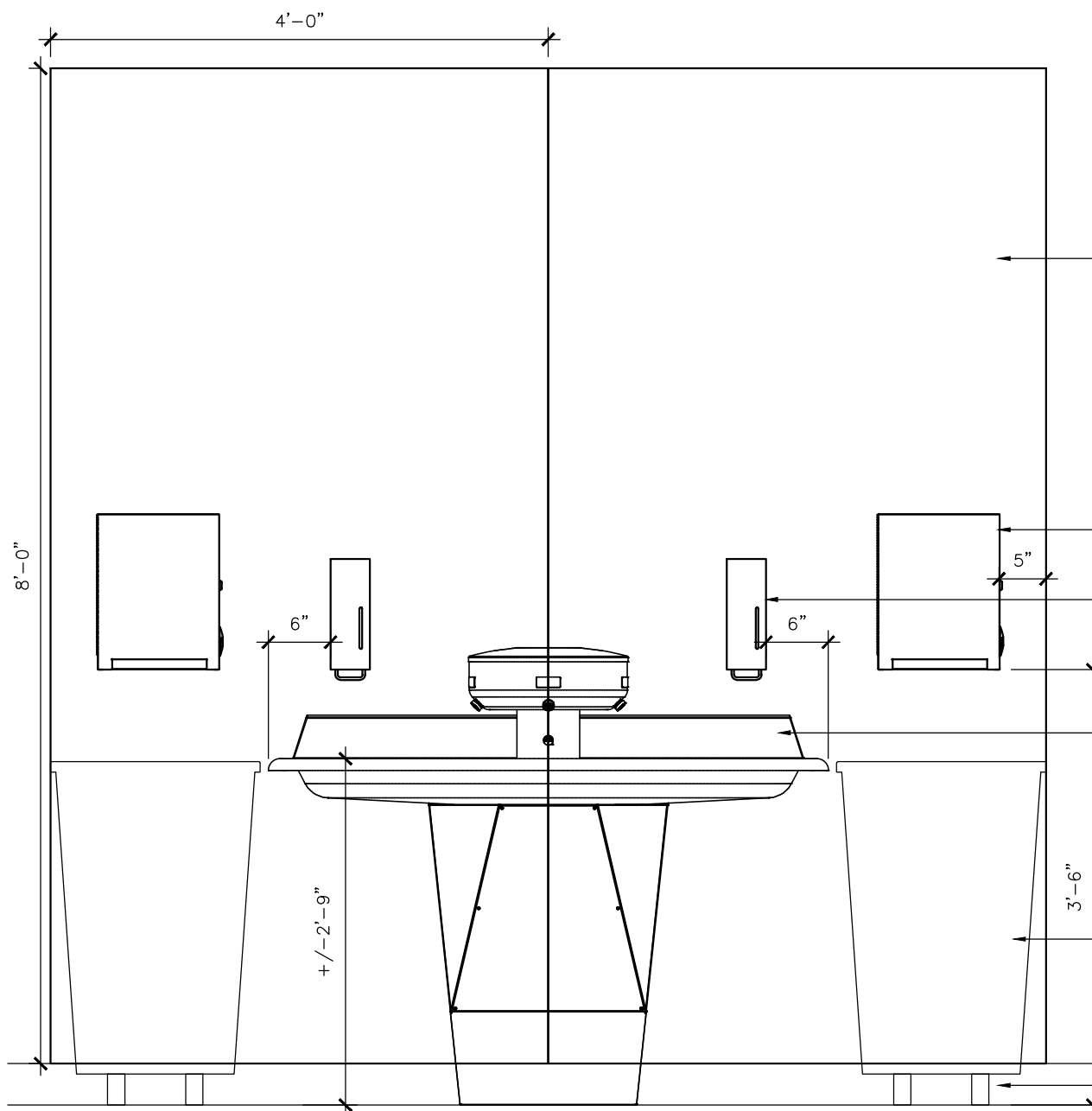
FRONT VIEW
